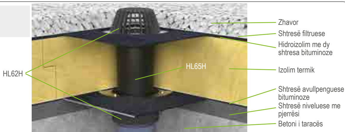
Taracë me zhavor
